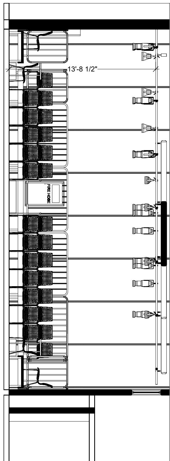
CENTERLINE SECTION
